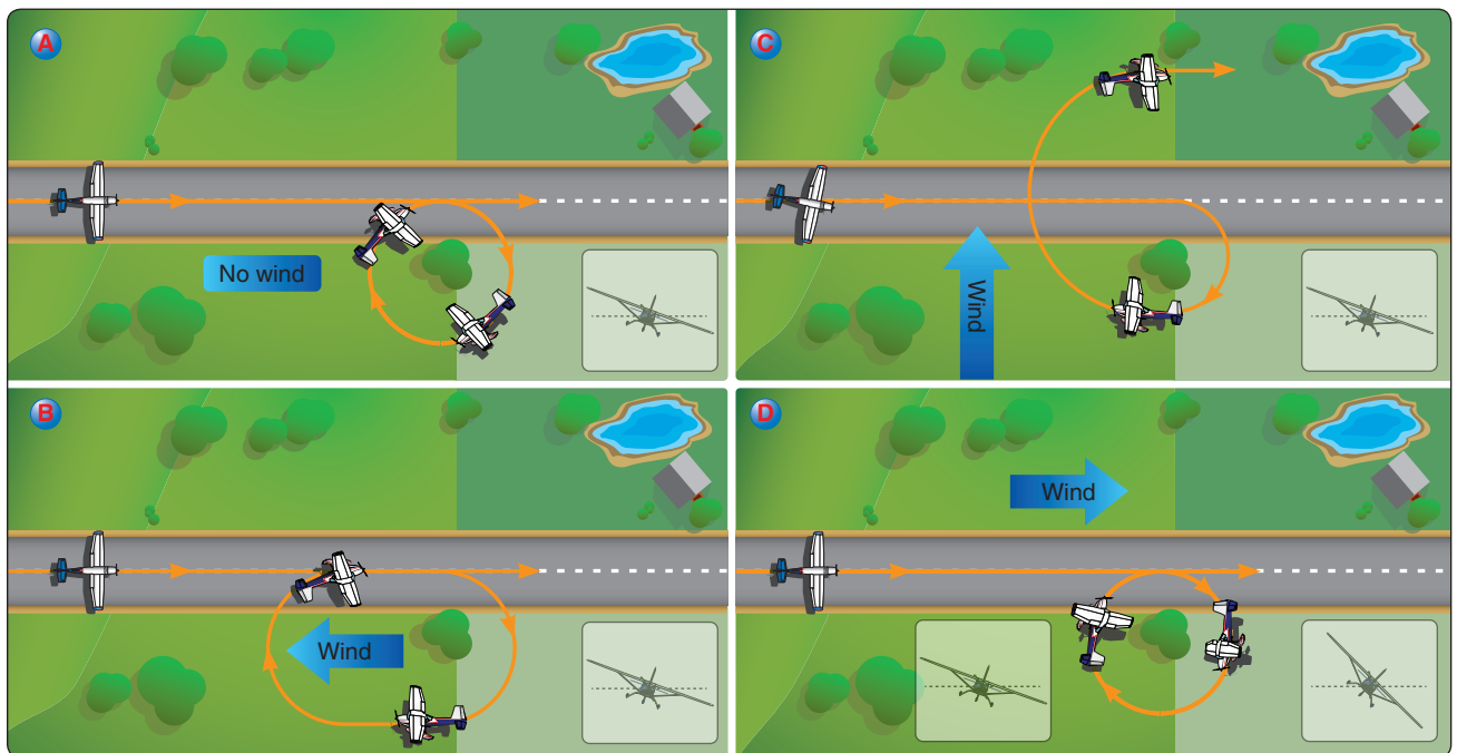
Figure 6-3. Effect of wind during turn.
