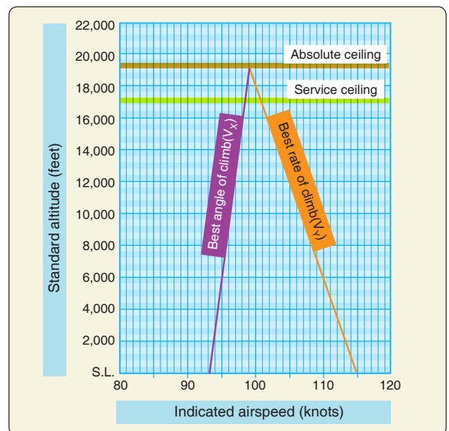
Figure 3-20. Absolute ceiling.
